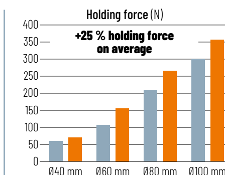
■ Standard suction cups ■ CTC Series
