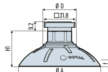
C32 Square coupling 32
