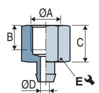
Female fittings VPAL 10...20
